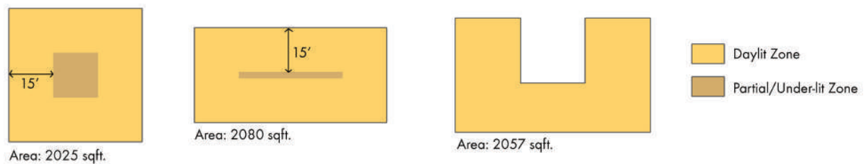
Figure 19: Daylit area for massing studies for different shapes of floor plan having similar floor area considering lintel level at 7 feet [6]
