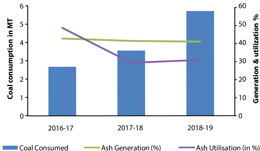
Figure 29: Generation and utilisation of fly ash, STPS
