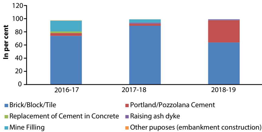
Figure 30: Fly ash consumption for various purposes, STPS
